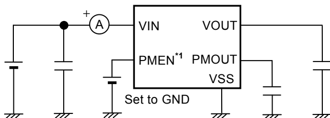
Figure 7 Test Circuit 2
