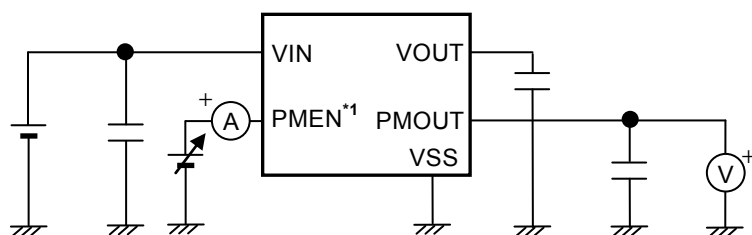
Figure 11 Test Circuit 6
