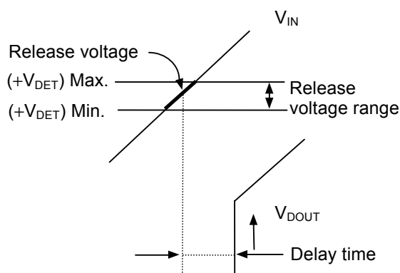
Figure 30 Release Voltage
