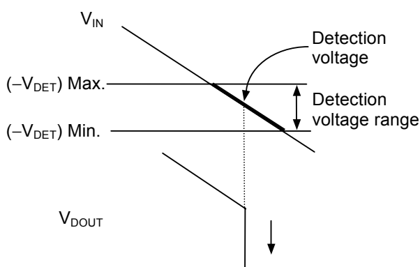
Figure 29 Detection Voltage
