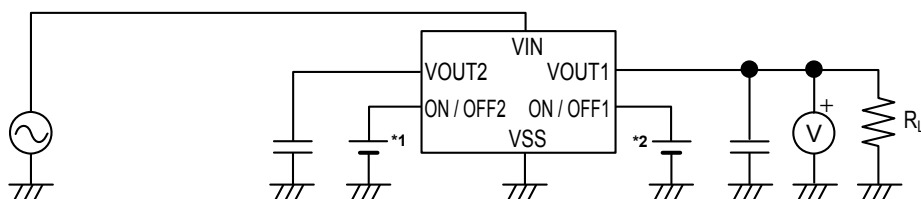
Figure 17 Test Circuit 7
