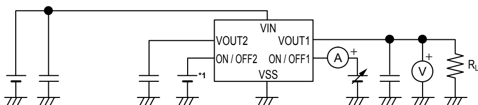
Figure 15 Test Circuit 5
