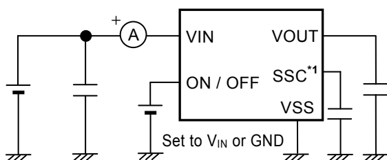
Figure 14 Test Circuit 2
