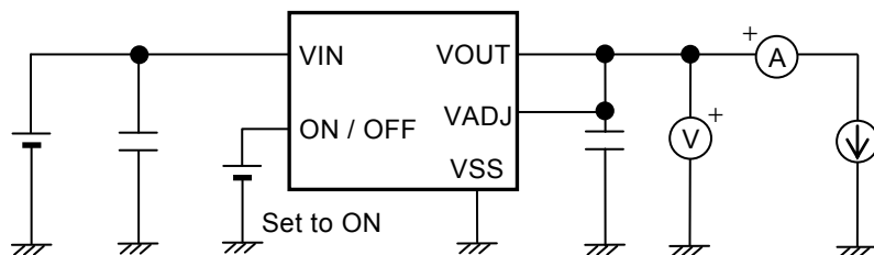
Figure 19 Test Circuit 7
