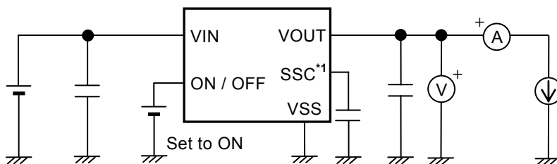
Figure 13 Test Circuit 1
