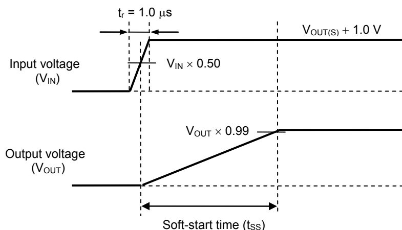
Figure 31 Basic Operation
