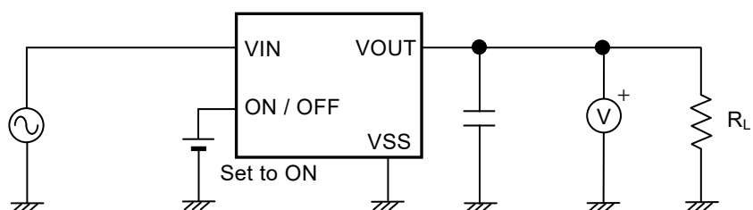
Figure 14 Test Circuit 5
