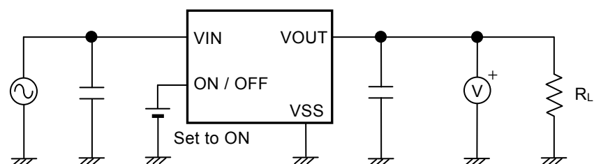
Figure 12 Test Circuit 5
