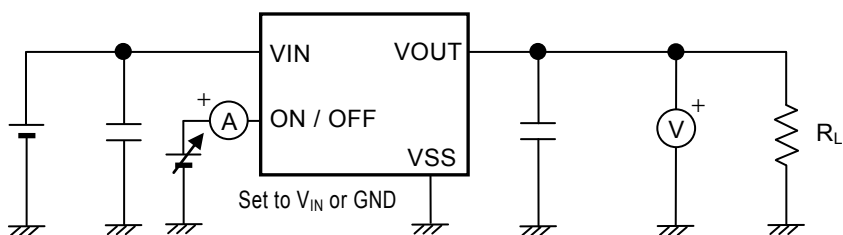
Figure 10 Test Circuit 4
