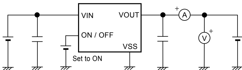
Figure 9 Test Circuit 3
