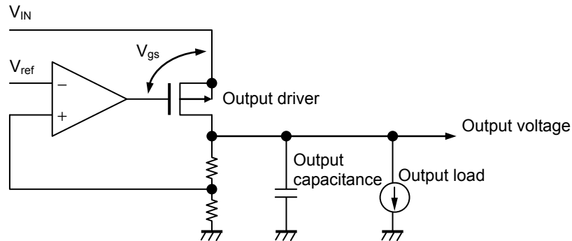
Figure 12 Circuit Diagram
