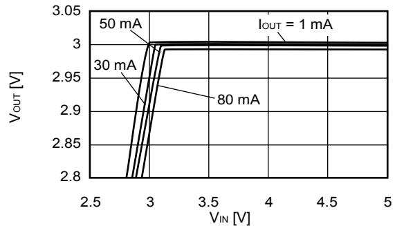
S-1131B30 ( T_a = 25^\circ\text{C} )
