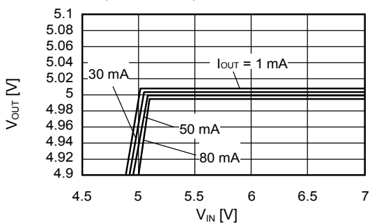
S-1131B50 ( T_a = 25^\circ\text{C} )
