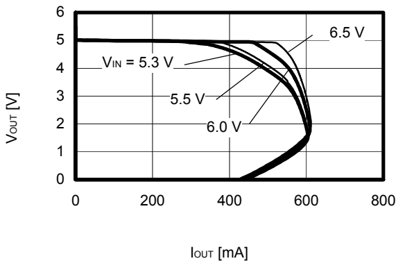
S-1131B50 ( T_a = 25^\circ\text{C} )
