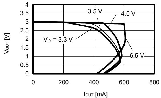
S-1131B30 ( T_a = 25^\circ\text{C} )
