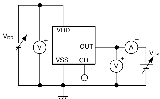
Figure 9 Test Circuit 3
