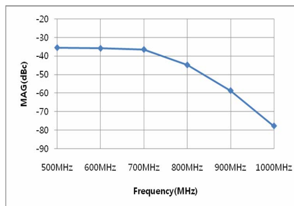
2 nd Harmonics
