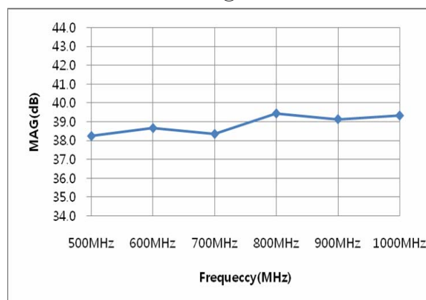
Power Gain @ Pin=8dBm
