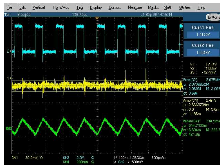
Figure 15. L=GLK2510P-2R2M, C=Ceramic 4.7μF 0805 X5R TDK (Ripple 12.4mV)
