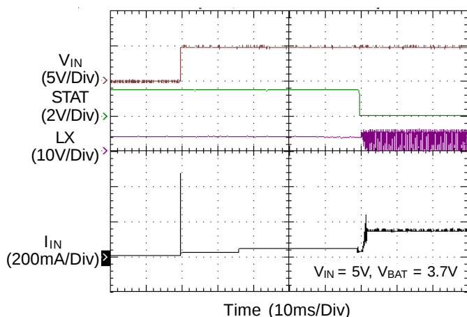
Adapter Insertion
