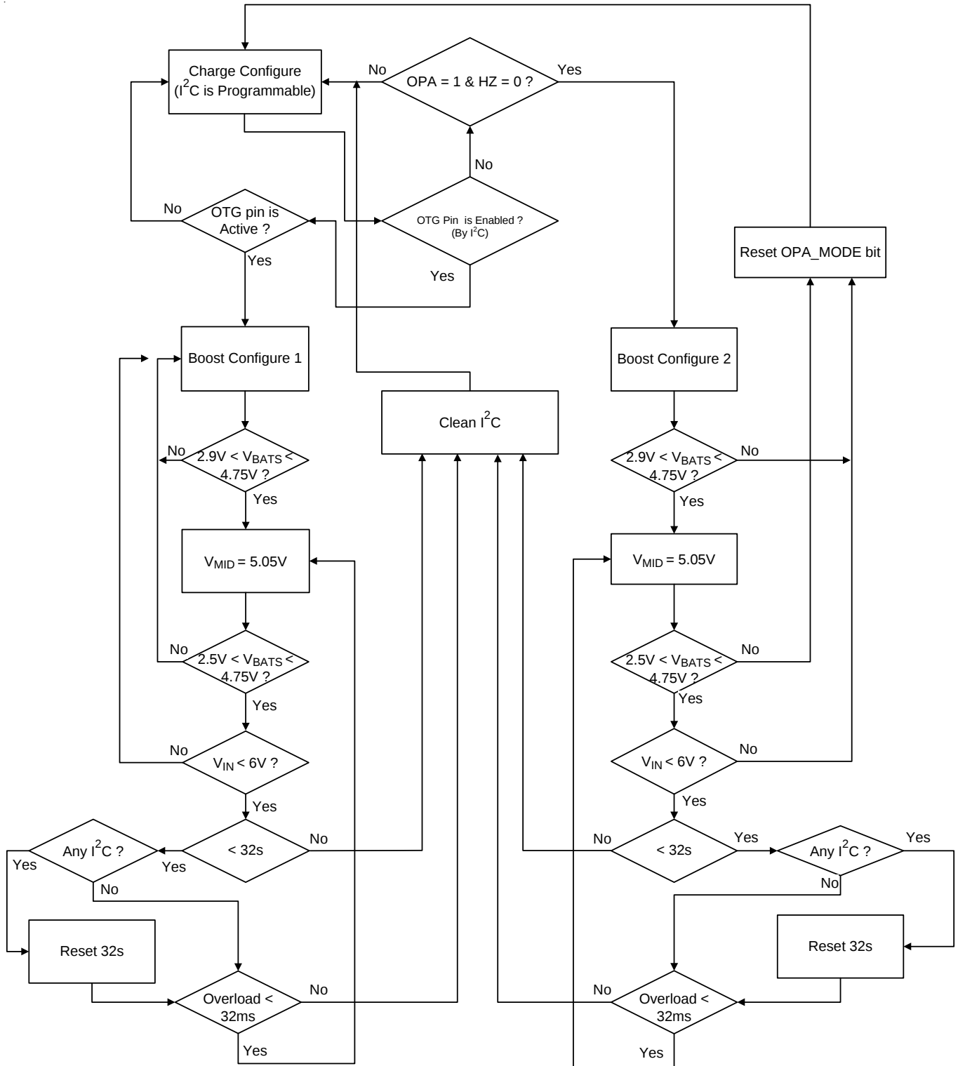
Figure 8. OTG Mode
