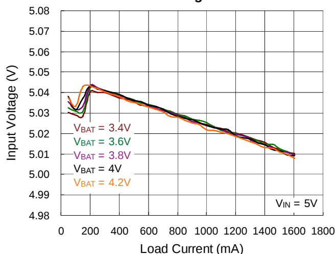
Load Regulation
