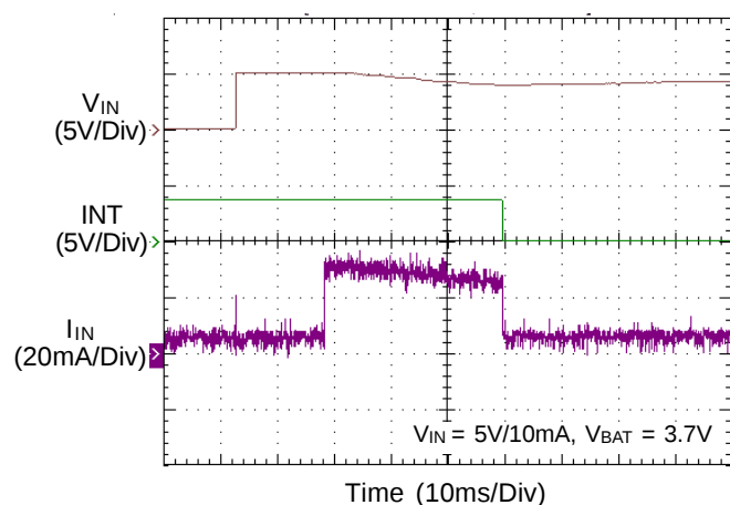
Bad Adapter
