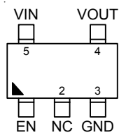
SOT-23-5/SC-70-5
