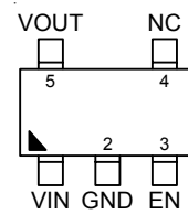
SOT-23-5/SC-70-5 (R-Type)
