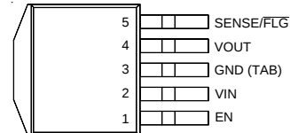
TO-263-5 RT9172N-□□xM5 RT9172F-□□xM5
