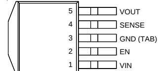
TO-263-5 RT9172S-□□CM5
