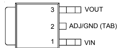
TO-252 (R-Type)
