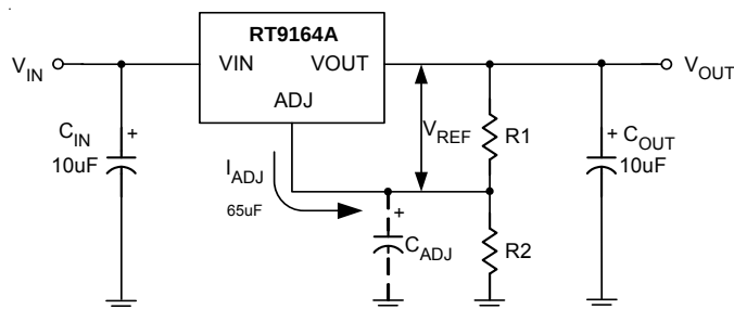
Figure 4. Basic Adjustable Regulator
