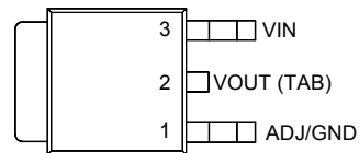
TO-252
