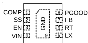
WDFN-8L 3x3
