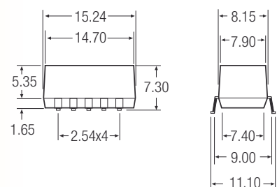
10 PIN Dual SMD Package
