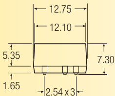
8 PIN SMD Package
