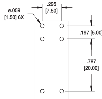
Recommended PCB Layout 2 Form A
