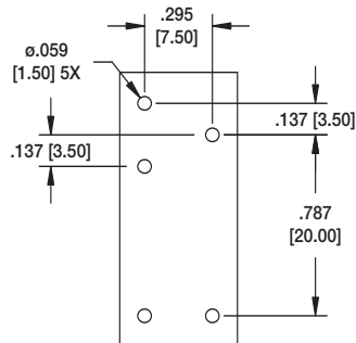
Recommended PCB Layout 1 Form C
