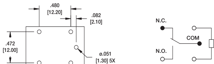
Schematic 1 Form C
