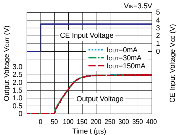
RP110x25xB/D
