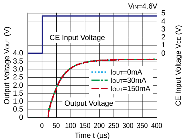
RP110x36xB/D
