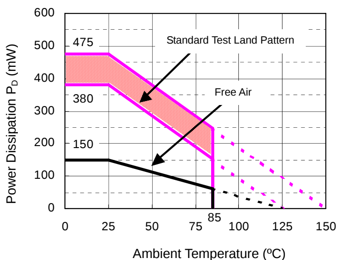
Power Dissipation
