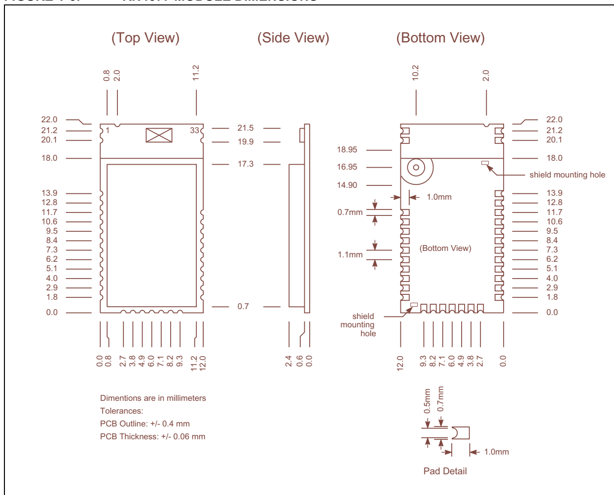
FIGURE 1-6: RN4677 MODULE DIMENSIONS
