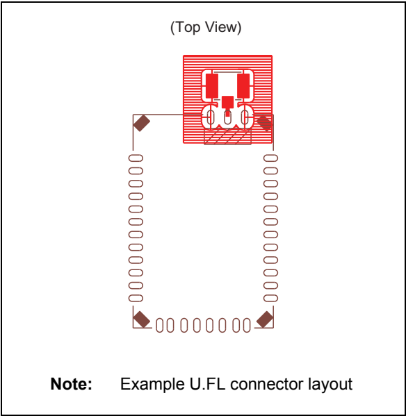
FIGURE 2-4: RN41N MODULE MOUNTING DETAILS
