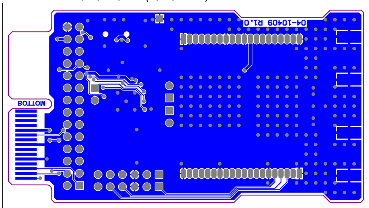
FIGURE A-4: RN2483 LORA™ TECHNOLOGY PiCtail™/PiCtail PLUS DAUGHTER BOARD BOTTOM COPPER (BOTTOM VIEW)
