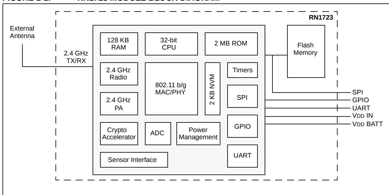
FIGURE 1-1: RN1723 MODULE BLOCK DIAGRAM
