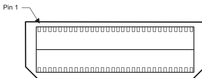
Figure 2-4. J19, 60 Pin MIPI ETM Header
