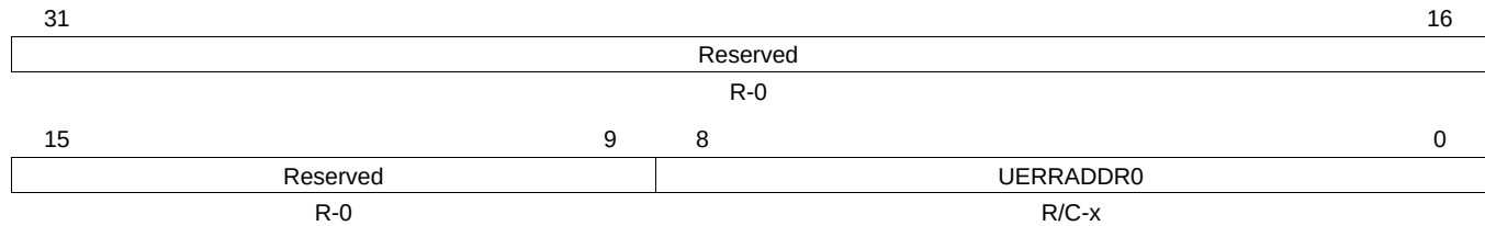
Figure 27-71. TXRAM Uncorrectable Parity Error Address Register (UERRADDR0) [offset = 12Ch]
