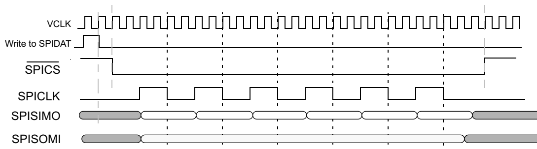
Figure 27-82. SPI/MibSPI Pins During Master Mode 4-pin with \overline{\text{SPIC}}\text{S} Configuration
