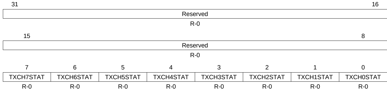
Figure 31-24. EMAC Control Module Transmit Interrupt Status Register (C0TXSTAT)
