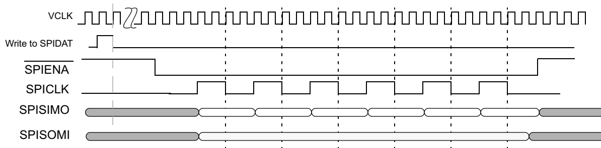
Figure 27-83. SPI/MibSPI Pins During Master Mode 4-pin with \overline{\text{SPIEN A}} Configuration
