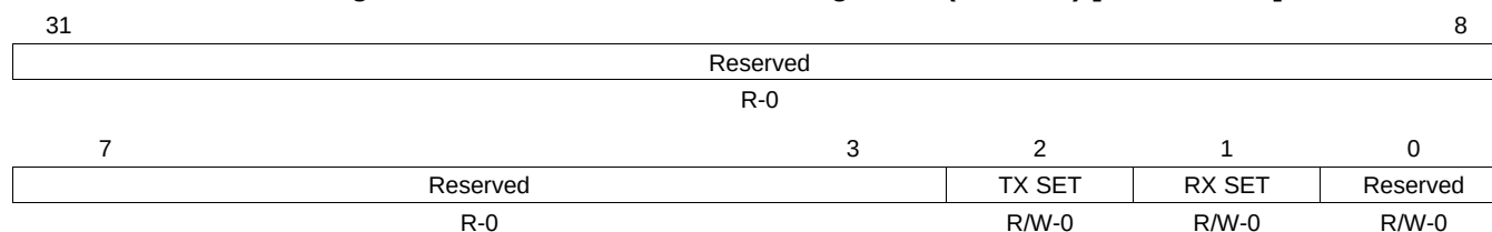
Figure 29-26. SCI Pin I/O Control Register 4 (SCIPIO4) [offset = 4Ch]
