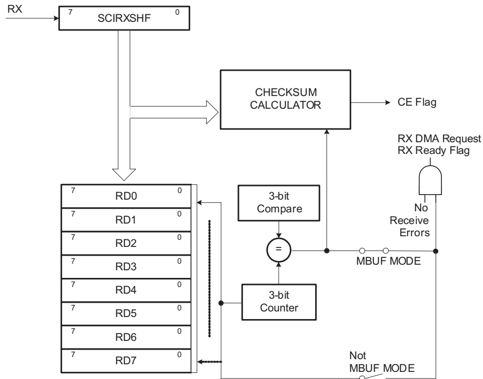
Figure 28-8. Receive Buffers
