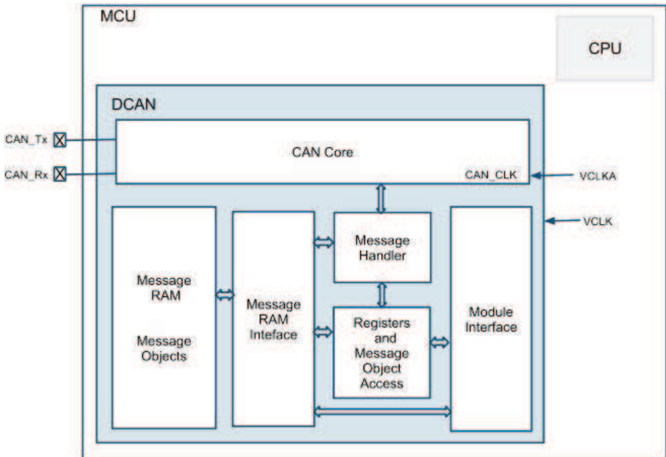
Figure 26-1. Block Diagram
