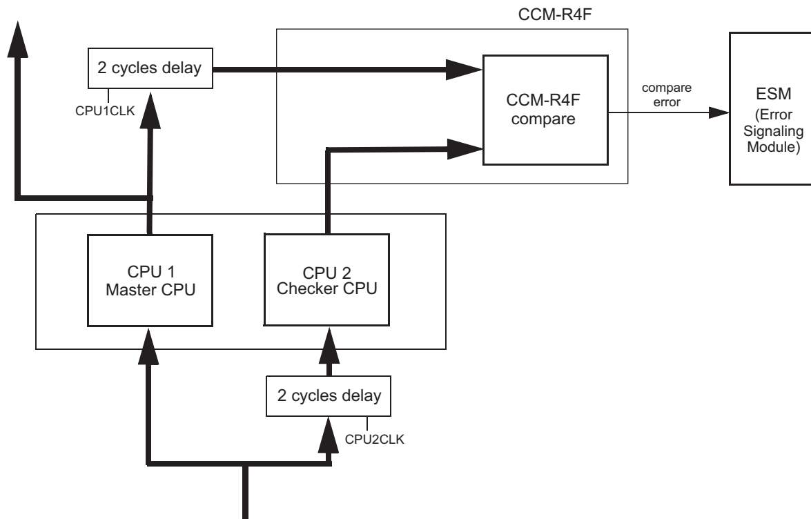
Figure 9-1. Block Diagram
