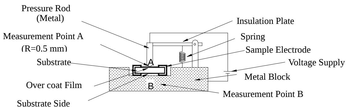
Figure 1 : Measurment Setup
