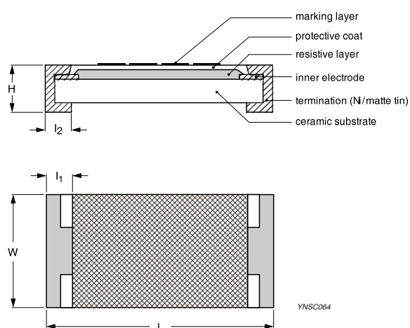
Fig. 4 Chip resistor outlines
