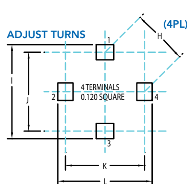
RECOMENDED LAND PATTERN
