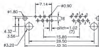
PCB Layout
