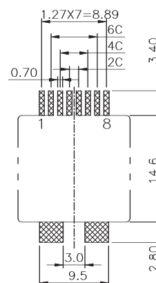
PCB Layout
