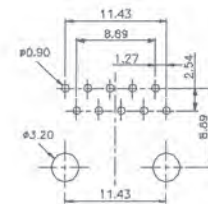
PCB Layout
