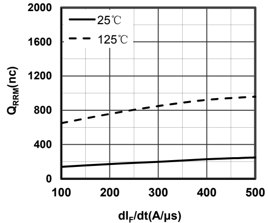
Figure 4. Reverse Recovery Charge vs dI_F/dt
