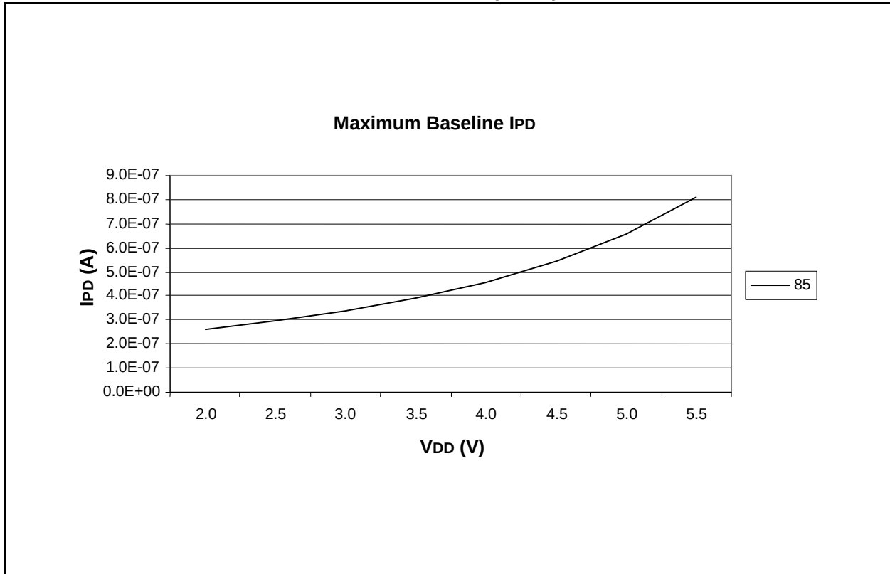
FIGURE 14-5: MAXIMUM I PD vs. V DD OVER TEMP (+85°C)
