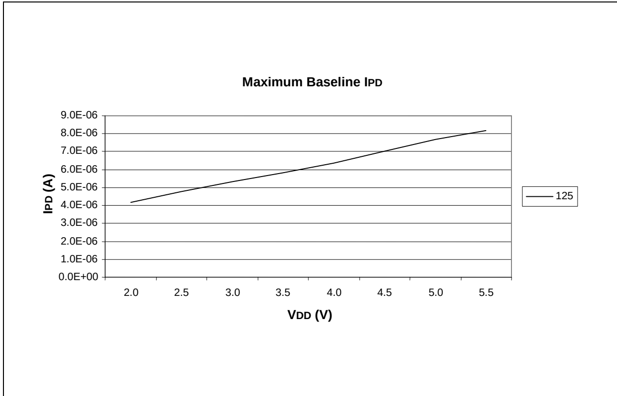
FIGURE 14-6: MAXIMUM I PD vs. V DD OVER TEMP (+125°C)
