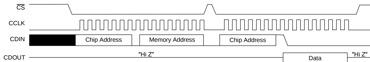
Figure 7. SPI Read Functional Timing Diagram
