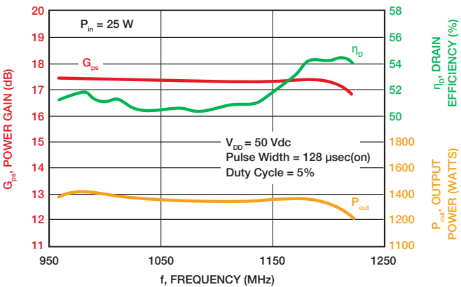
Power Gain, Drain Efficiency and Output Power versus Frequency
