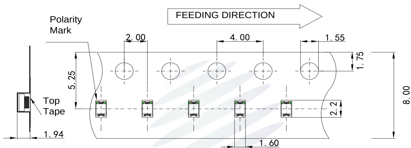
Fig.2-1 Carrier Tape Dimension 載帶尺寸
