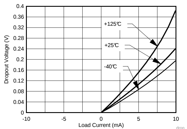
Dropout vs Current Load Over Temperature
