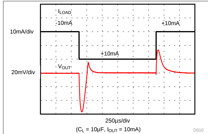
Figure 13. Load Transient
