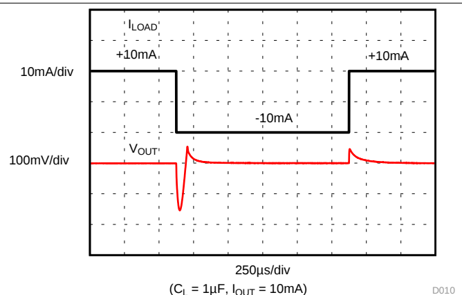
Figure 10. Load Transient
