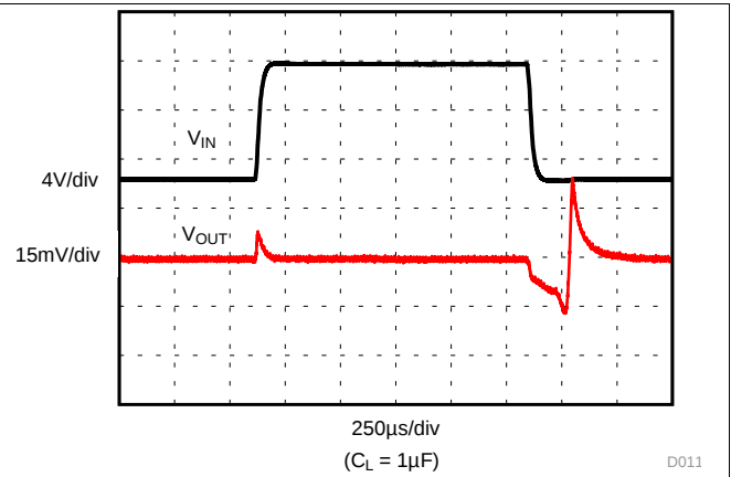
Figure 14. Line Transient
