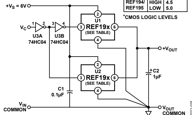
Figure 30. Switched Output Reference
