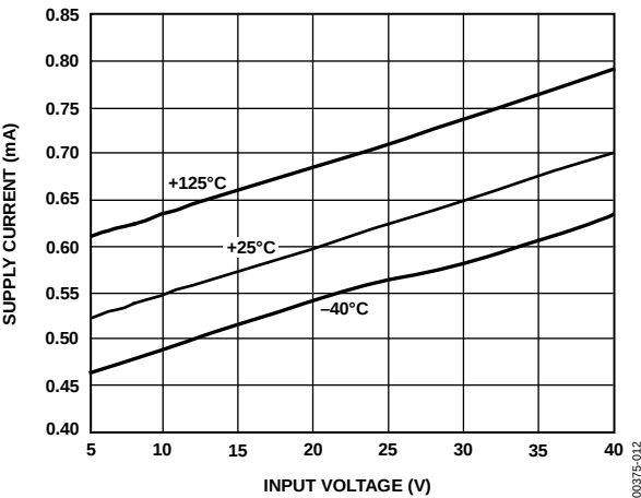
Figure 12. REF03 Supply Current vs. Input Voltage
