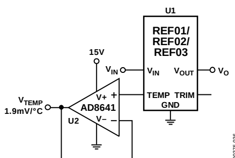
Figure 36. Temperature Monitoring
