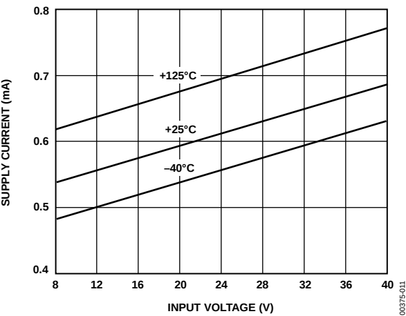
Figure 11. REF02 Supply Current vs. Input Voltage
