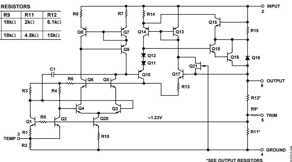
Figure 4. Simplified Schematic
