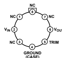
Figure 1. TO-99 (J-Suffix)
