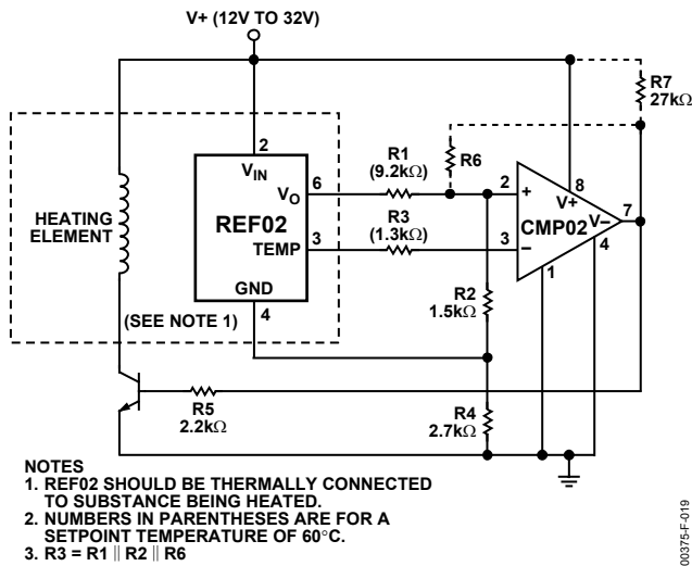
Figure 20. Temperature Controller
