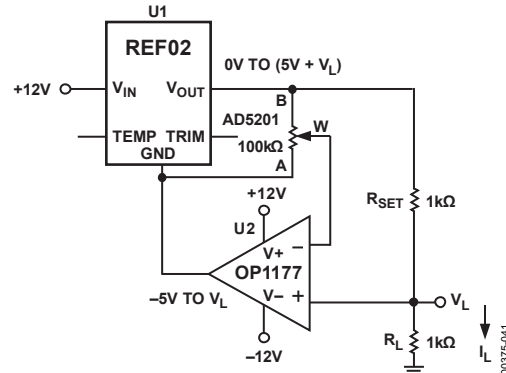
Figure 40. Programmable 0 mA to 5 mA Current Source
