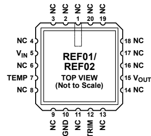
Figure 2. 8-Lead TO-99 (J-Suffix)
