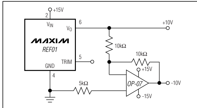
Figure 3. ±10V Reference
