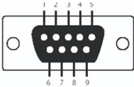
DB9 connector
