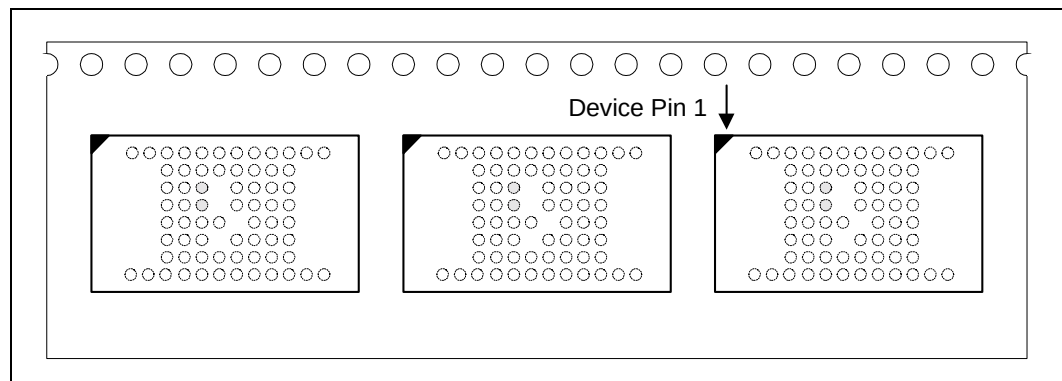
Figure 23. Stacked-CSP Device in 24 mm Tape (8 mm x 10 mm and 8 mm x 12 mm)
