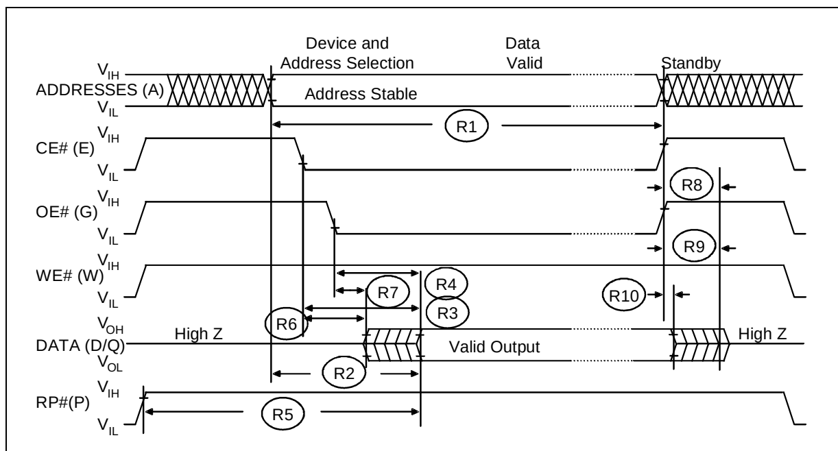
Figure 6. AC Waveform: Flash Read Operations
