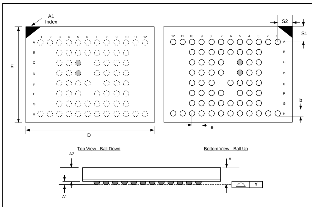
Figure 21. Stacked-CSP: 12 x 8 Ball Matrix
